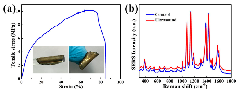
Figure 2. (a) Stress–strain curve of the Au@Ag@Au-NCs/PVC film. (inset) Digital photographs of the Au@Ag@Au-NCs/PVC film wrapping around a glass rod and folded by hand. (b) SERS spectra of 4-ATP collected from the Au@Ag@Au-NCs/PVC film before and after ultrasonication. Experimental conditions: laser power = 0.04 mW; integration time = 10 s.
