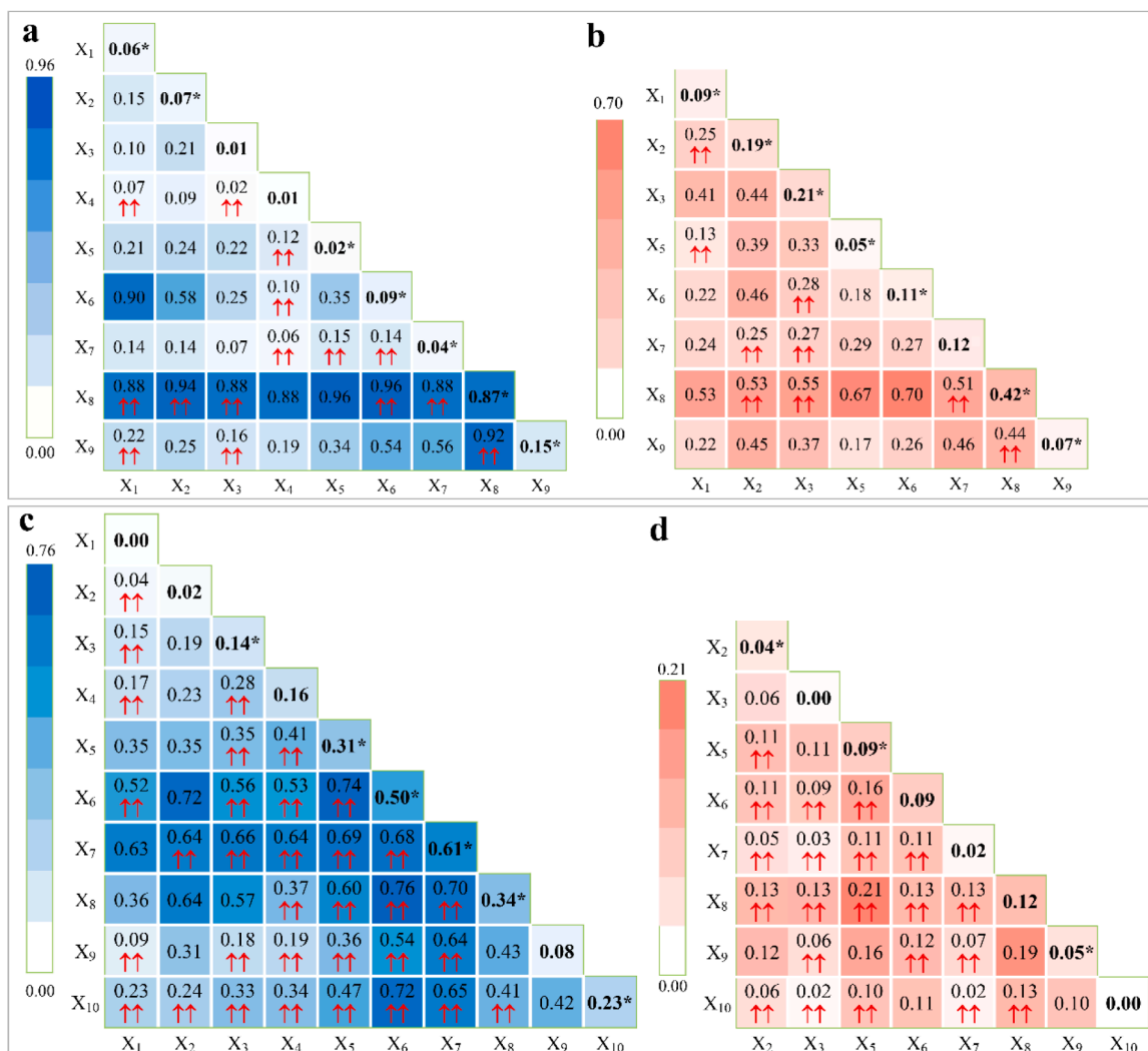
Fig. 4. Driving forces of microplastic abundance (a and b) and relative abundance of small-sized microplastics (c and d) in waters (a and c) and sediments (b and d). The q -values on diagonal line are driving forces of individual factors, and "*" represent 5% significance levels. The larger the q -values, the greater the influence degree of dependent variable by factor or interaction. Left triangular matrix shows q -values for interaction pairs of factors. "↑↑" means that two-factors enhanced each other. The rest are nonlinear enhancement. Factors: X 1 – longitude, X 2 – latitude, X 3 – sampling location relative to the reservoir, X 4 – sampling depth, X 5 – land-use type, X 6 – seasonal variation, X 7 – sampling method, X 8 – extraction method, X 9 – identification method, X 10 – microplastics abundance.
