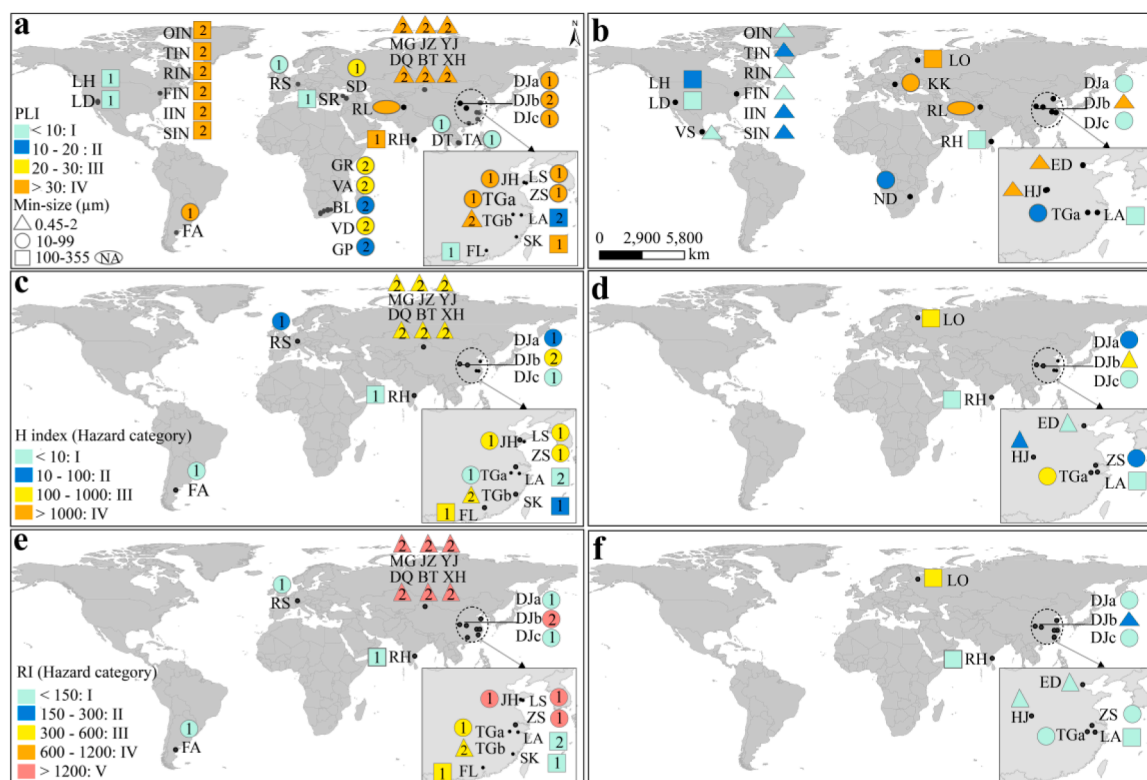
Fig. 7. Risk of microplastics pollution in reservoirs. Pollution load index ( PLI ) in waters (a) and sediments (b); (b) Polymer risk assessment index ( H index) in waters (c) and sediments (d); (c) Potential ecological risk index ( RI ) in waters (e) and sediments (f). Different shapes represent different orders of magnitude of the minimum collection size (Min-size). The ellipse indicates Min-size unknown. Values in the boxes indicate sampling methods of microplastics. Sampling methods: 1 – volume-reduced sampling method, 2 – bulk sampling method.
