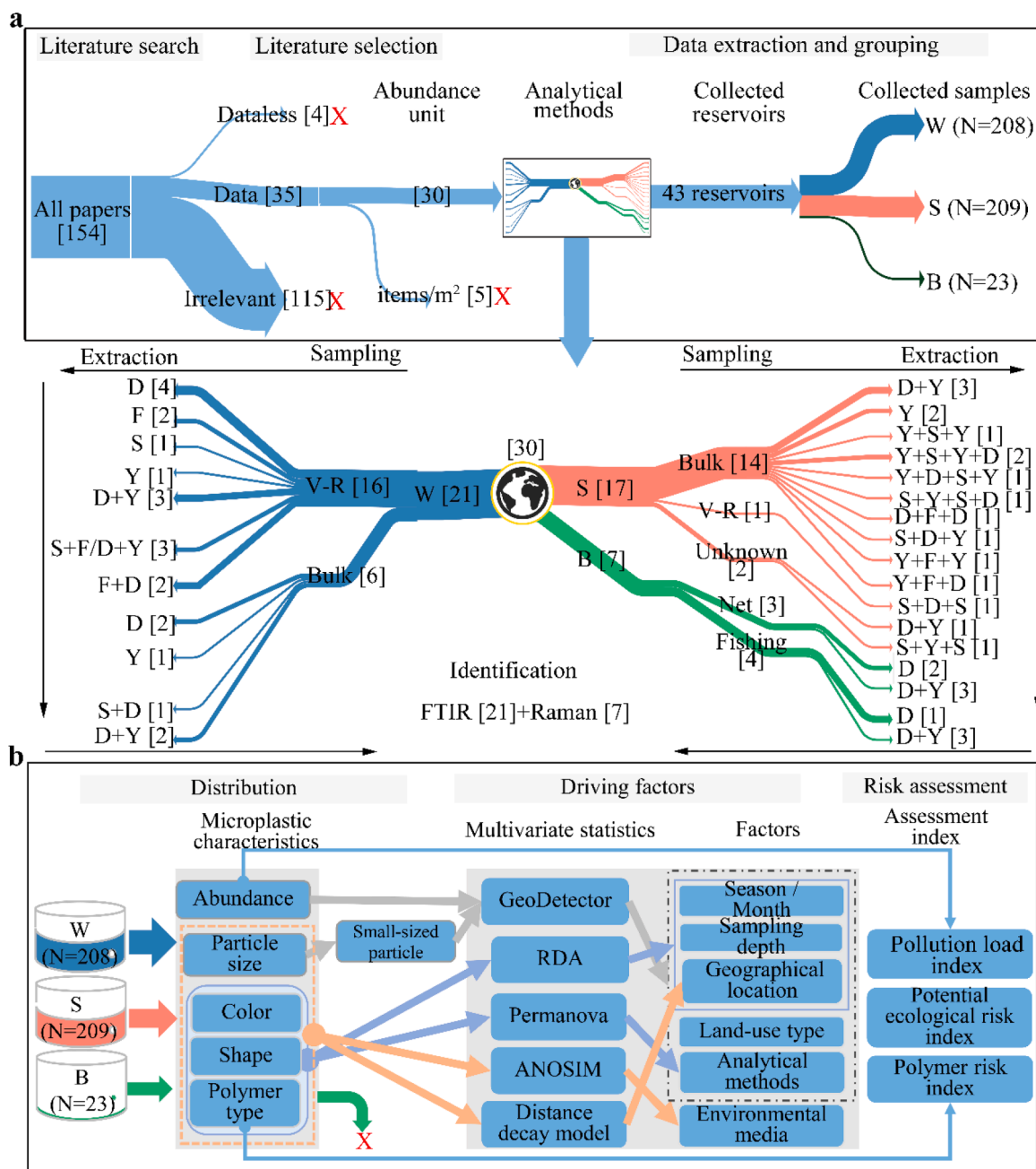
Fig. 1. A schematic representation of our literature search and Data processing and Multivariate statistics for extraction of data for the systematic review and meta-analysis. (a) Data processing. A red "X" indicates that article or data was excluded. Environmental media: W – Waters, S – Sediments, B – Biota. The values after environmental media represent the number of samples. V-R and Bulk represent two sampling methods of collecting waters and sediments: volume-reduced sampling and bulk sampling method; D, F, S and Y represent four sample extraction methods: digestion, filtration, sieving and density separation, respectively. Samples were extracted and then filtered through membranes for visual identification and spectroscopic analysis of microplastics. Among the analytical methods, there were studies that used multiple sampling methods or investigated multiple environmental media, resulting in a total number of studies that exceeded thirty. (b) Multivariate statistics. Small-sized particle is defined as microplastics with particle size < 1 mm.
