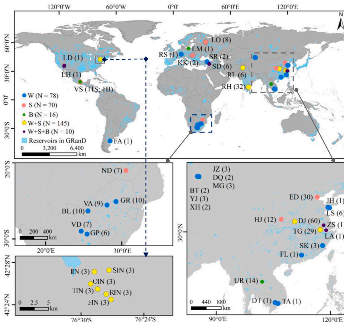
Fig. 2. Distribution map of samples for microplastics in reservoirs (from 43 reservoirs in 30 studies). The letters and numbers next to samples are the abbreviated name of reservoir and the number of microplastic sampling sites, respectively (Table S1). Blue dots are water samples (W); Orange are sediment samples (S); Green are biotic tissue samples (B); Yellow are water and sediment samples collected simultaneously (W + S); Black represent water, sediment, and biotic tissue samples collected simultaneously (W + S + B).
