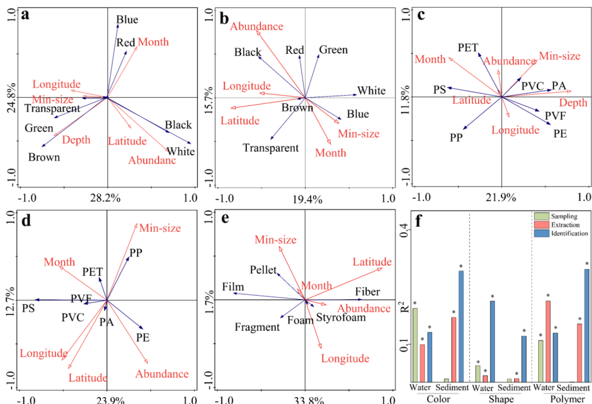
Fig. 6. Redundancy analysis (RDA) of common colors (a and b), polymer types (c and d), and shapes (e) of microplastics with explanatory variables in waters (a and c) and sediments (b, d and e). (f) Permutational multivariate analysis tests (Permanova) tests explanation degree ( R^2 ) for differences in color, shape, and polymer type of microplastic by analytical methods. Marked "*" represents 5% significance level and unmarked indicates results at significant level of p > 0.05 .
