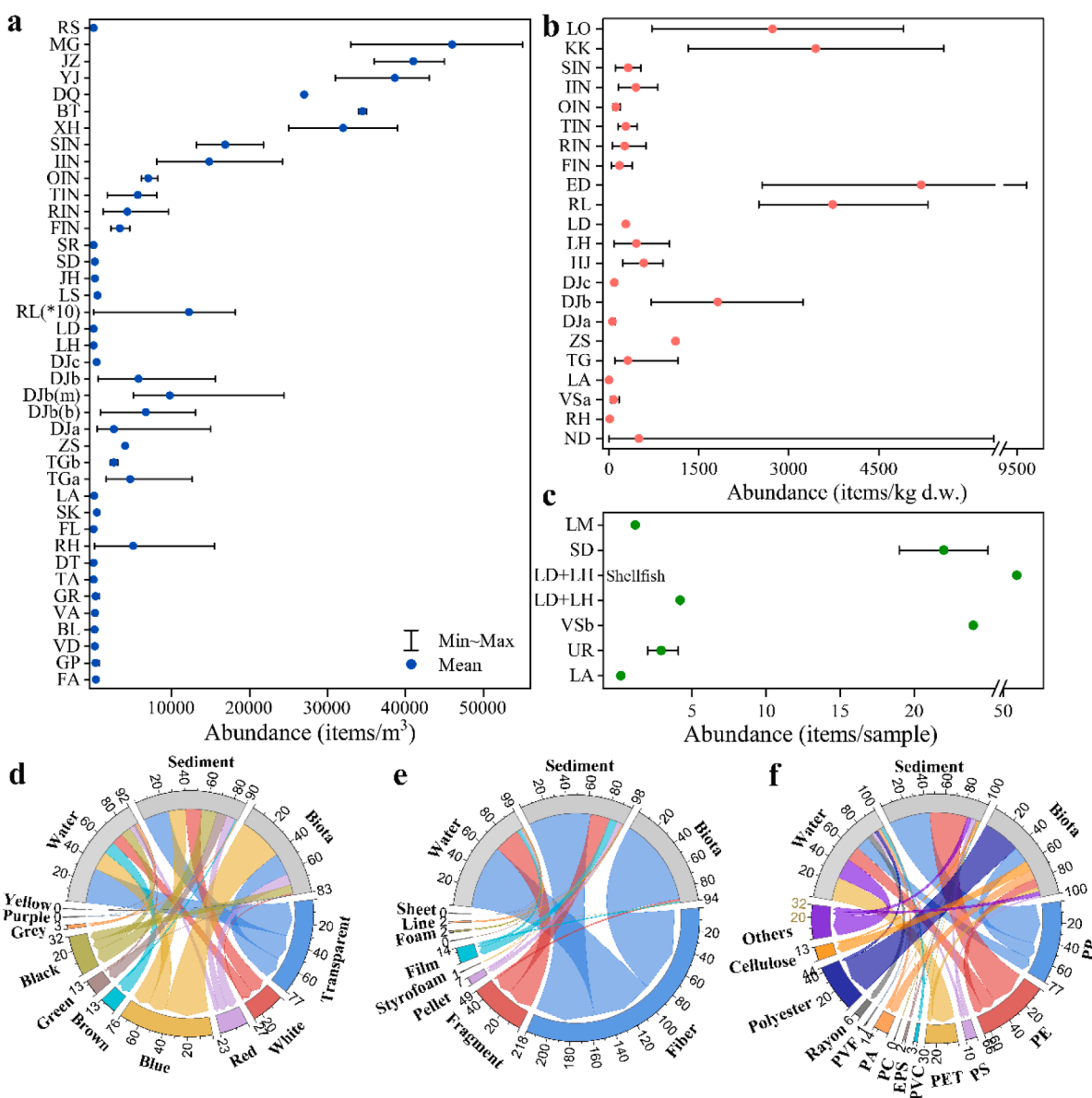
Fig. 3. Microplastic abundances in waters (a), sediments (b) and biota (c) of reservoirs. Distribution of color (d), shape (e) and polymer type (f) of microplastics in waters, sediments, and biota samples. The lowercase letters a , b , and c were marked after the abbreviated names of reservoirs in order to distinguish the order of the detection time. "(m)" and "(b)" represent water samples collected in the middle and bottom layer, respectively. The remaining unlabeled ones are surface waters. Values on the chord diagram are the percentages of microplastic characteristics.
