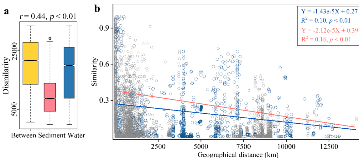
Fig. 5. Differences of microplastic morphological characteristics in waters and sediments (a). Distance decay of microplastic characteristics similarity (1-Bray-Curits) versus geographic distance in waters and sediments (b). The line indicates regression line.
